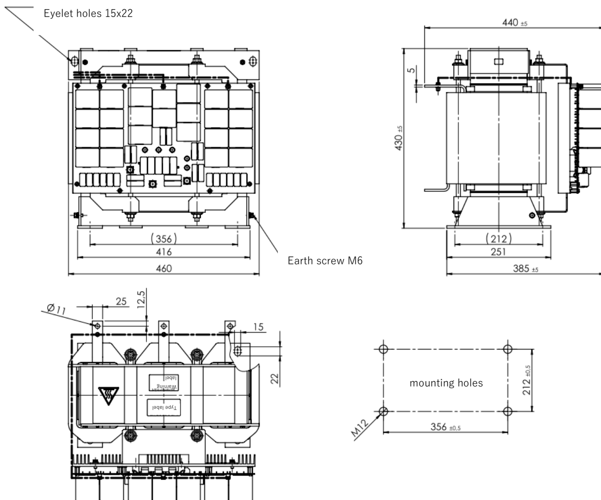
Picture 3-6 Technical drawing dv/dt filter MTZEF051-26
